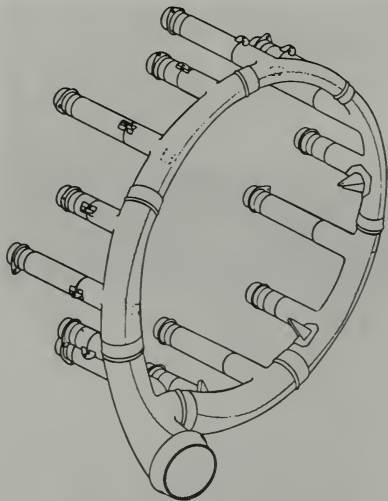
FIGURE 2-31. Exhaust collector ring.
